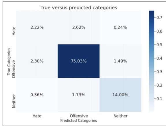
Figure 4: Results of BERT finetuned on 4chan data on Davidson dataset
