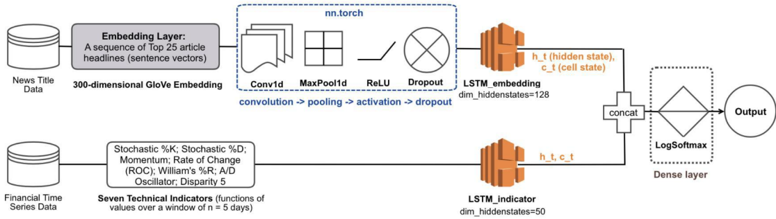
Figure 1: RCNN Baseline Model Architecture
