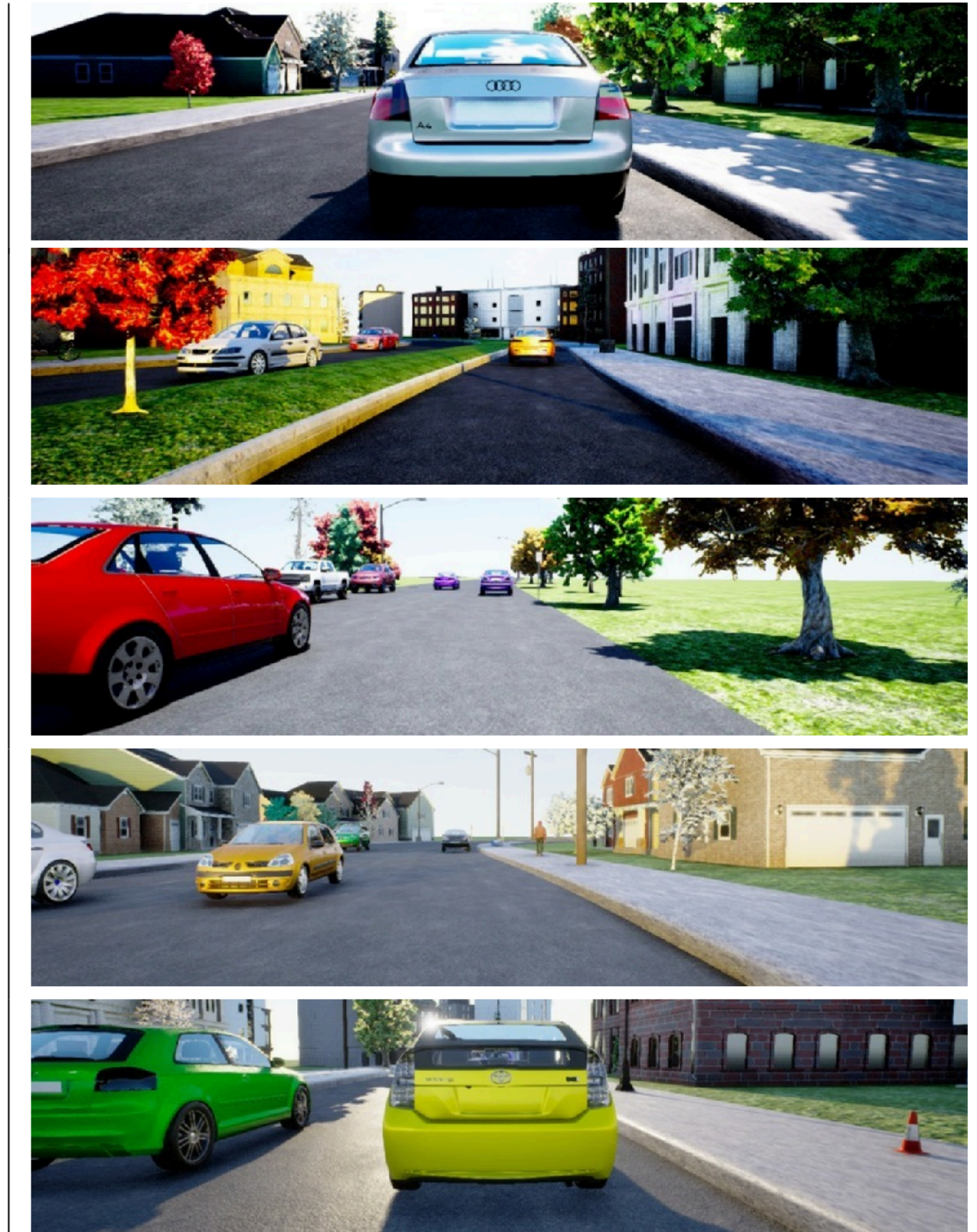
After Meta-Sim
