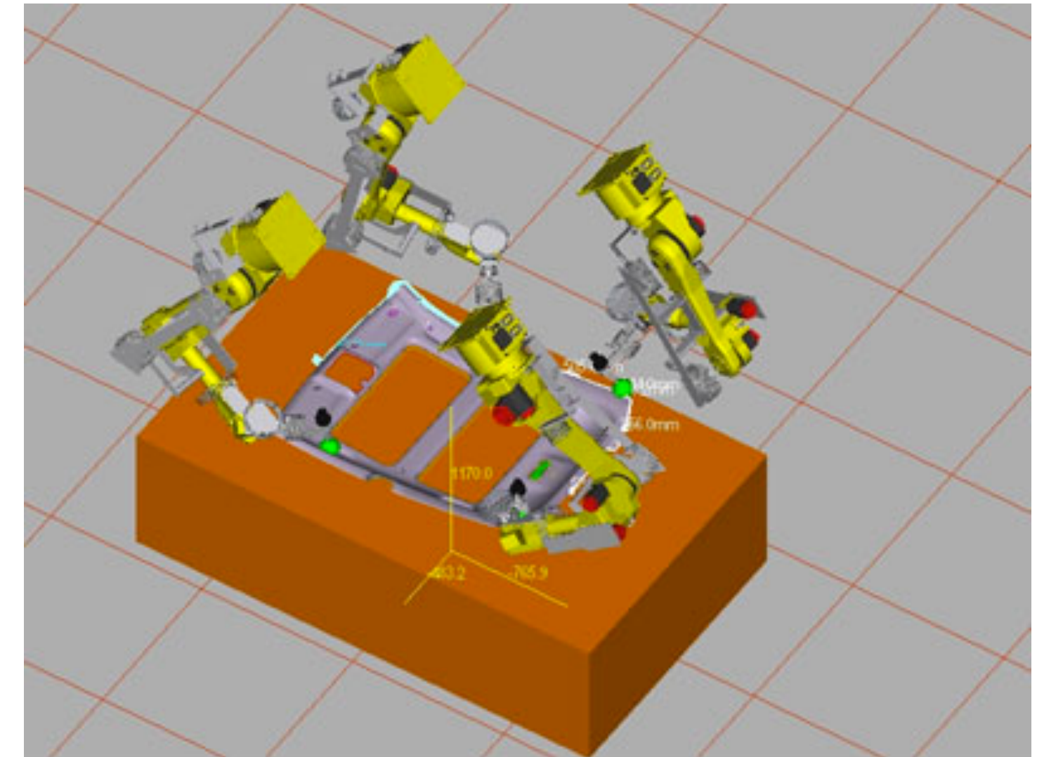
Simulation of robotic headliner trimming, courtesy KMT Robotic Solutions Inc.
