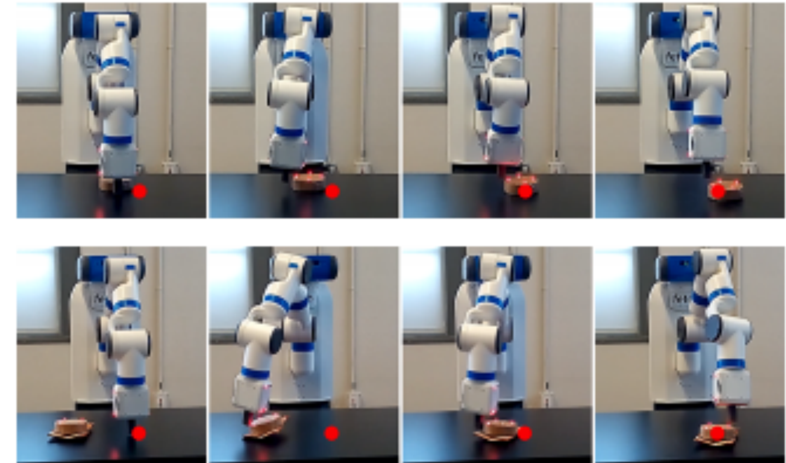
Fig. 3. LSTM policy deployed on the Fetch arm. Bottom: The contact dynamics of the puck was modified by attaching a packet of chips to the bottom.
